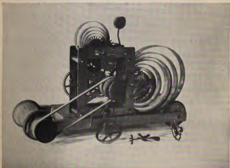
FIG 161. THE FRAMEWORK.
